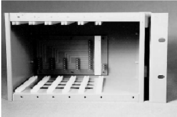
6A09 Bracket shown with 6A02 Rack
